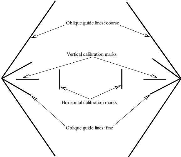
Figure 2. Calibration chart of the linear stereo set-up
