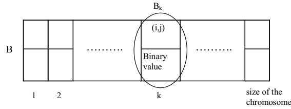
Figure 10. Binary chromosome
