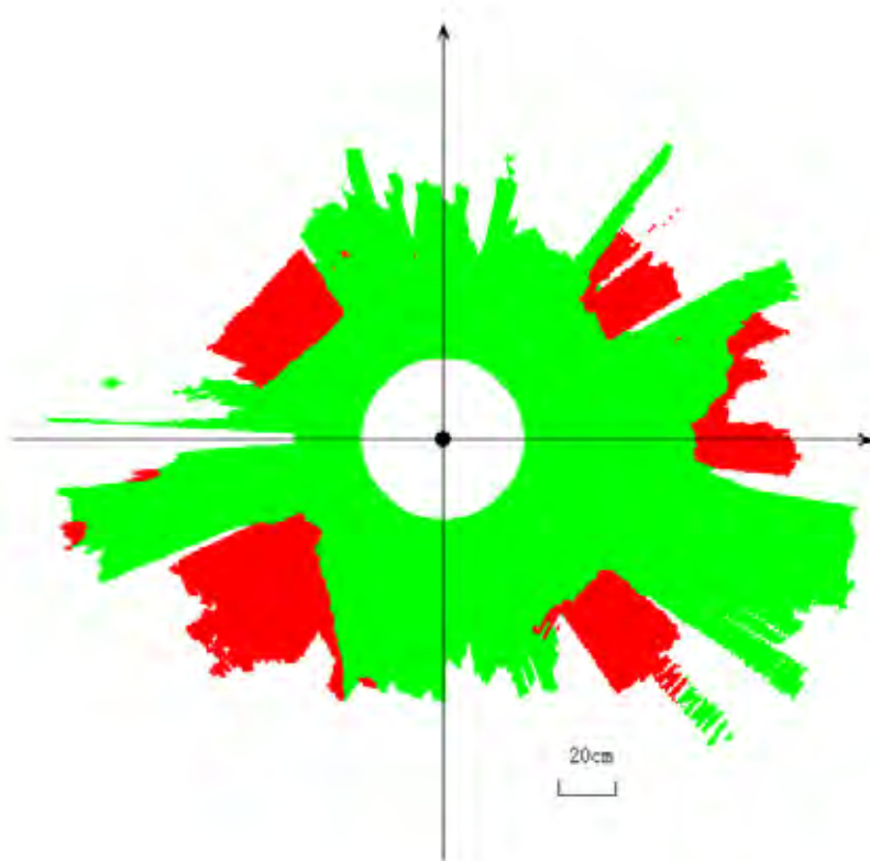
Figure 10. Omnidirectional scene information obtained by our system, of which green represents navigable areas, red detected obstacle areas
