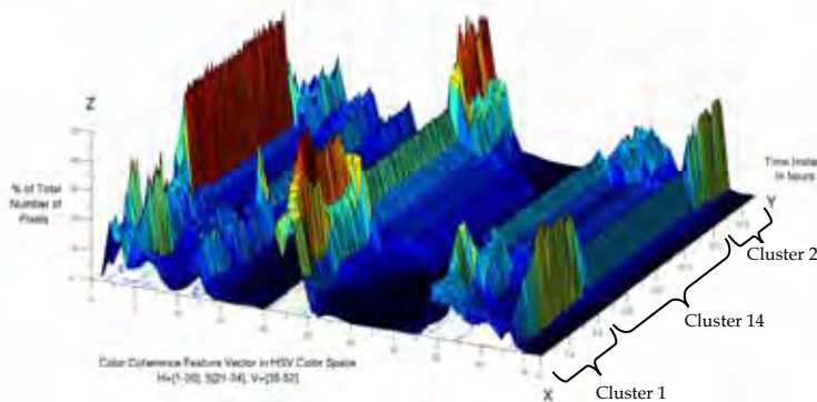
Figure 17. 3-D histogram of the image sequence used during the experiment (see Figure 3 for samples). Each X-Z slice is an histogram which represents the percentage of the number of pixels (Z axis) belonging to a given color coherent feature (X axis). The coherent color feature scale has been divided into 3 intervals for the three HSV channels. Histograms are ordered along the Y axis which represents the time in the course of a day. Several clusters of histograms can be easily visually discriminated as notified for cluster number 1, 14 and 2. Others clusters not represented here are intermediate ones and mainly correspond to transitions states between the three main clusters
