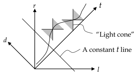
Figure 6. An epipolar slice of the match space. The matching surface appears as a curve here. The monotonicity constraint means that this curve crosses every constant t line once.
