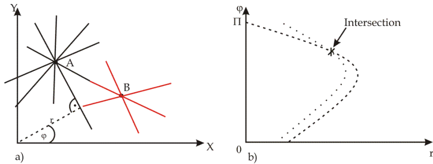
Figure 14. Hough transform a) Line bundle in the X, Y system b) Line bundle in the r, \varphi system
