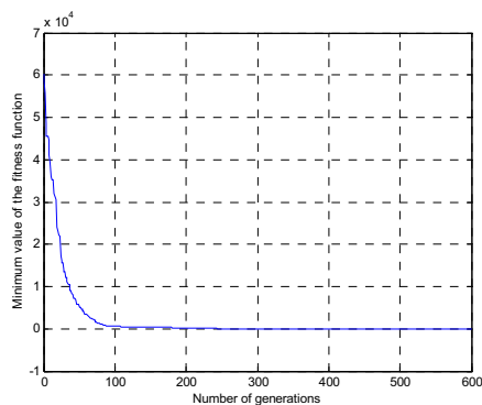
Figure 16. Evolution of the fitness function using the binary genetic algorithm, with a population of 300 chromosomes and 600 generations
