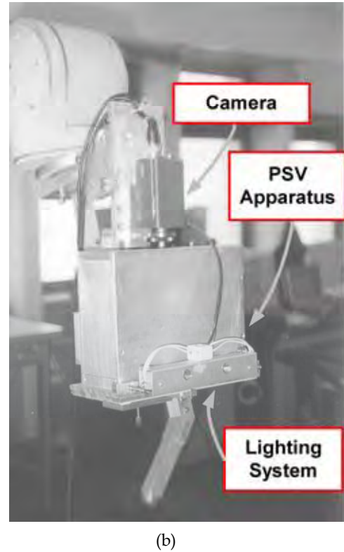
Figure 1. PSVS: (a) Mirrors position (b) PSV apparatus mounted on the end effector of a PUMA 761 robotic manipulator
