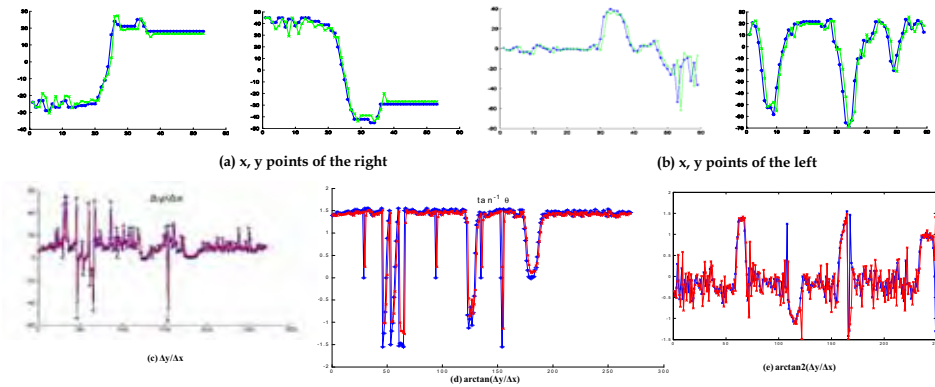
Figure 1. Learning and prediction accuracy using auto-regressive second-order model. Blue line stands for the original data and green and red lines are predicted data by AR2 model
