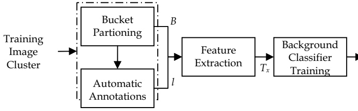
Figure 8. Background classifier training schema for figure-ground segmentation. Since training image sets are composed of only background images, the annotation task is fully automatic
