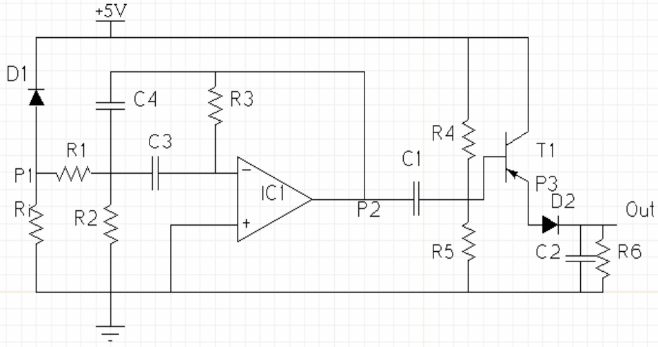
Fig. 11. A custom filter for high frequency carrier.
