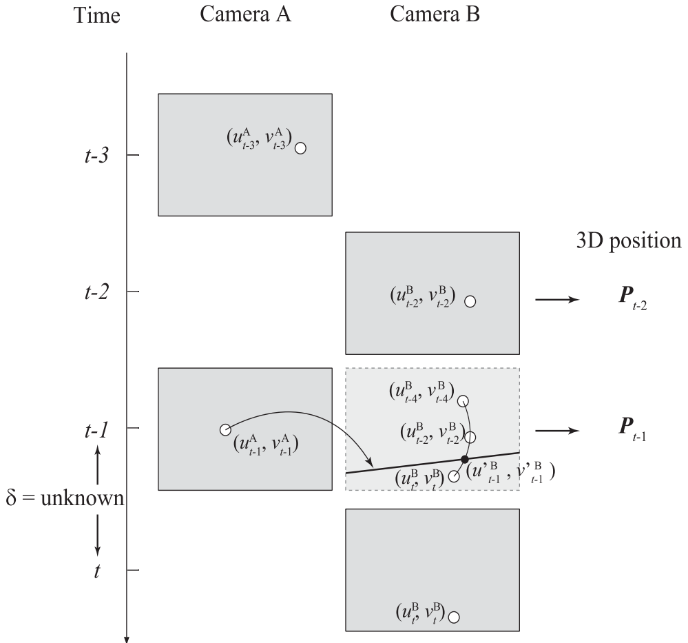
Figure 4. 3D position is estimated using spline curve
