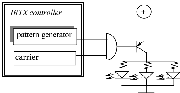
Fig. 2. The architecture of the IRTX device
