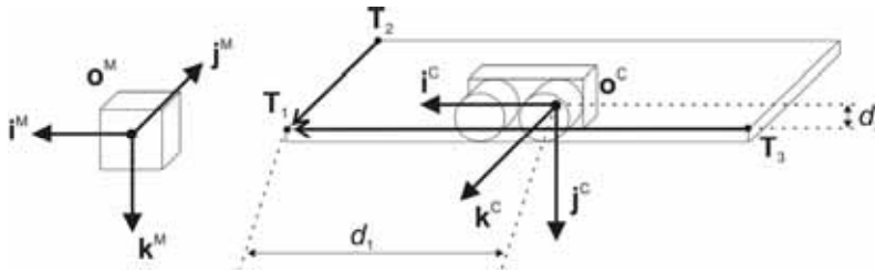
Figure 2. The setup of the magnetic tracker (left) and the camera (right) for model A. Vectors i^M , j^M , k^M denote base vectors of CS^M , while i^C , j^C , k^C denote base vectors of CS^C . T_1 , T_2 and T_3 mark the control point positions, while d_1 and d_2 mark manual measurements
