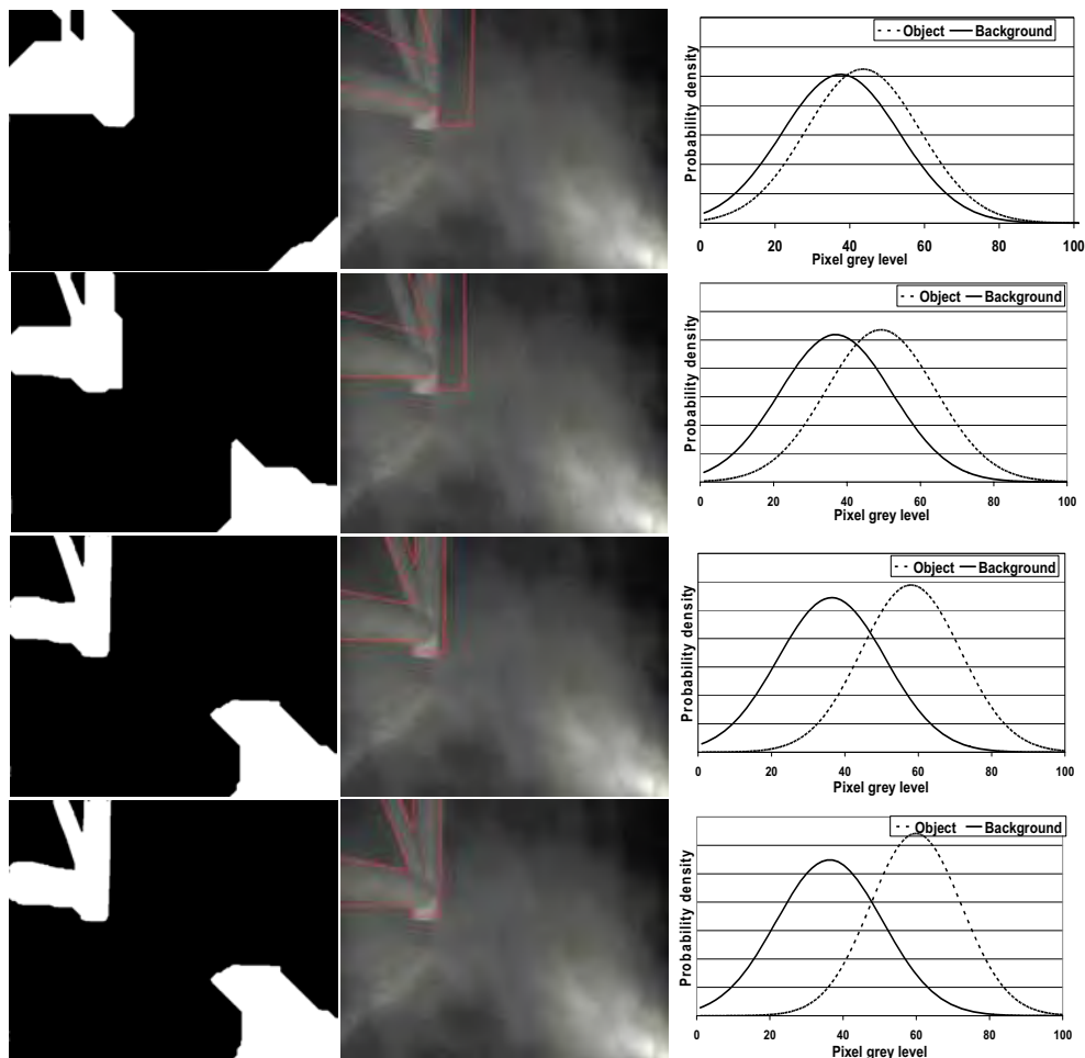
Figure 8. Example of EM/E-MRF tracking on a poor visibility image. Difficult, turbid conditions, encountered with underwater robotics, have been simulated in the lab with dry ice fog and focussed beam spot lights, mounted on and moving with the camera, leading to severe backscattering. Over four iterations, the EM/E-MRF algorithm homes in on an oil-rig like structure. Note how the algorithm mutually refines image interpretation, camera/object pose and the Gaussian object and background models. The two Gaussians separate as the algorithm progressively learns that object is relatively bright whereas background is relatively dark.
