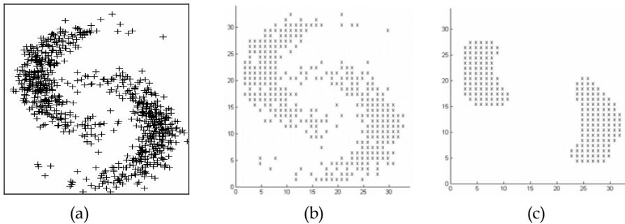
Figure 11. Mode detection by means of Markov Field Model
