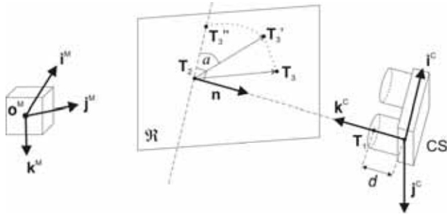
Figure 5. The setup of the magnetic tracker and the camera for model C. Vectors \mathbf{i}^M , \mathbf{j}^M , \mathbf{k}^M denote base vectors of CS^M , while \mathbf{i}^C , \mathbf{j}^C , \mathbf{k}^C denote base vectors of CS^C . T_1 , T_2 and T_3 mark the original control point positions, T_3' and T_3'' mark recalculated position of T_3 , while d denotes the lens' focal length. Plane \mathfrak{R} is perpendicular to the left optical axis
