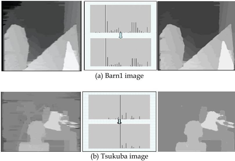
Figure 2. The result of disparity calibration (left: stereo matching result, middle: histogram comparison, right: calibrated disparity map)
