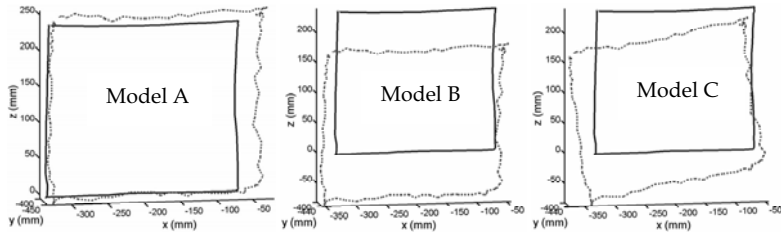
Figure 8. An example of transformation of vision-based trajectories from CSC to CSM , for each transformation model. The magnetic tracker data is depicted by solid lines, the video-based tracking algorithm data is depicted by dotted lines
