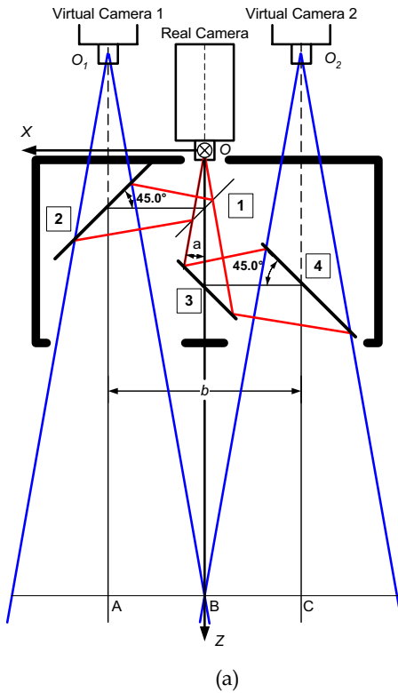
Figure 1. PSVS: (a) Mirrors position (b) PSV apparatus mounted on the end effector of a PUMA 761 robotic manipulator
