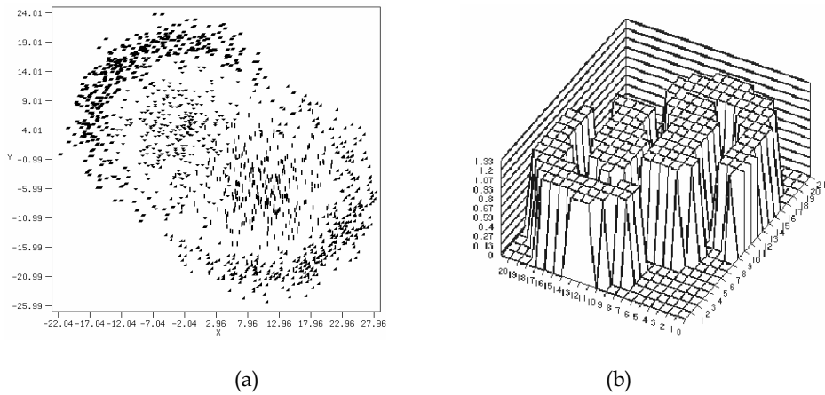
Figure 8. Mode detection for a bidimensional data set
