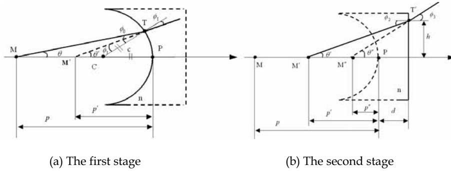
Figure 9. Refraction through the concave lens
