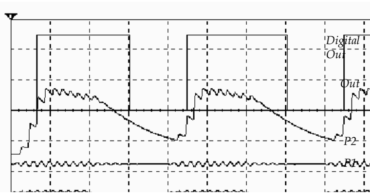
Fig. 12. The form of the received 1MHz signal at various stages of the MFBF filter.
