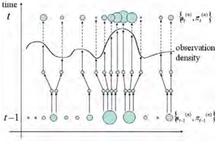
Figure 8. One time-step in particle filtering. There are 3 steps, resampling-diffusion-observation.
