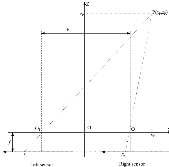
Figure 3. Pin-hole lens model
